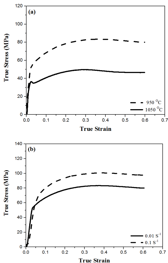
Fig. 1. True stress-strain curves of deformed specimens: a) at constant strain rate of 0.01 \text{s}^{-1} and b) at constant temperature of 950 °C.
