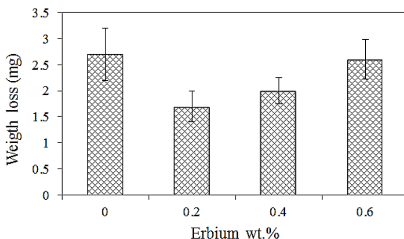
Fig. 10. The values of weight loss of samples with different concentrations of erbium.
