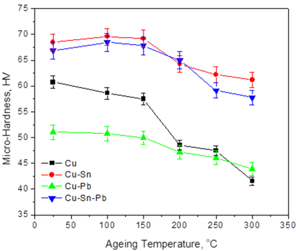
Fig. 1. Micro-hardness of sample materials against isochronal ageing temperature while aged for 1 hour.
