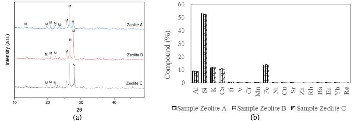
Fig. 2. a) XRD patterns of natural zeolite used in this study b) compounds found in natural zeolite used in this study
