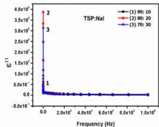
Fig. 5 Dielectric dissipation (Loss) plot for TSP-NaI at different wt.% ratios
