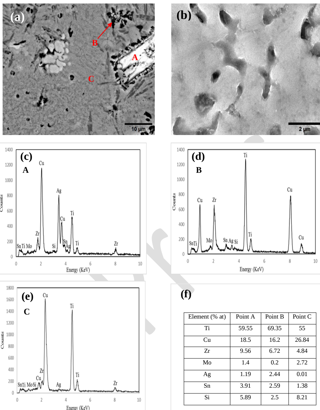
Fig2. Electron microscope image of different alloys a) \text{Ti}_{50}\text{Zr}_{15}\text{Cu}_{20}\text{Mo}_7\text{Ag}_4\text{Sn}_3\text{Si}_1 and b) \text{Ti}_{50}\text{Zr}_{25}\text{Cu}_5\text{Mo}_{10}\text{Ag}_6\text{Sn}_3\text{Si}_1 , c-f) EDS analysis of different areas in the \text{Ti}_{50}\text{Zr}_{15}\text{Cu}_{20}\text{Mo}_7\text{Ag}_4\text{Sn}_3\text{Si}_1 alloy
