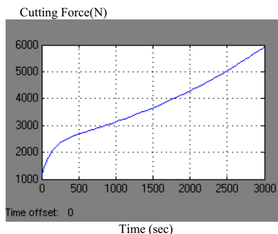
Fig. 11. Simulated cutting force diagram for a worn drill: diameter 15.9 mm, point angle 118°, helix angle 33°, pilot hole diameter 3.2 mm, speed 200 rpm, feedrate 0.102 mm/rev
