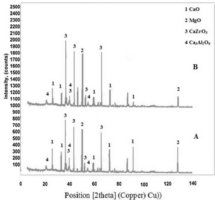
Fig. 4. XRD patterns of samples contain A) 2 wt. % and B) 8 wt. % ZrO 2 .
