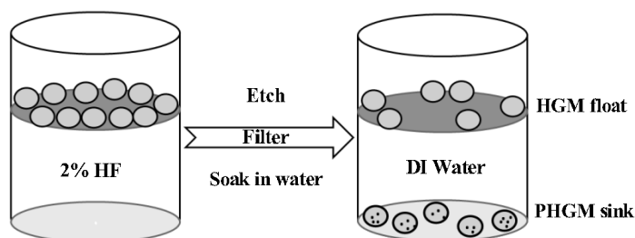
Fig. 1. Schematic of etching HGM to PHGM.
