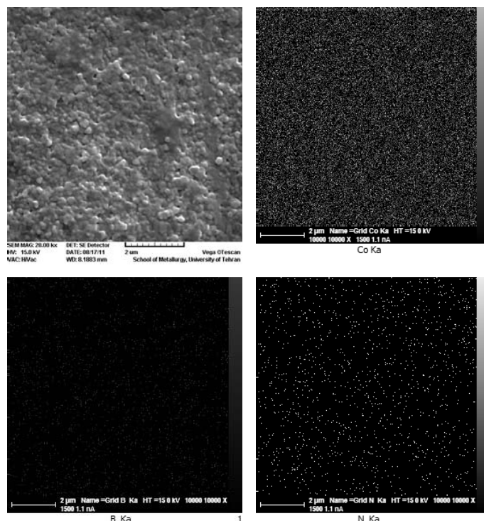
Fig. 1. SEM and EDS analysis of Co-BN (4 wt%) nano composite coatings.
