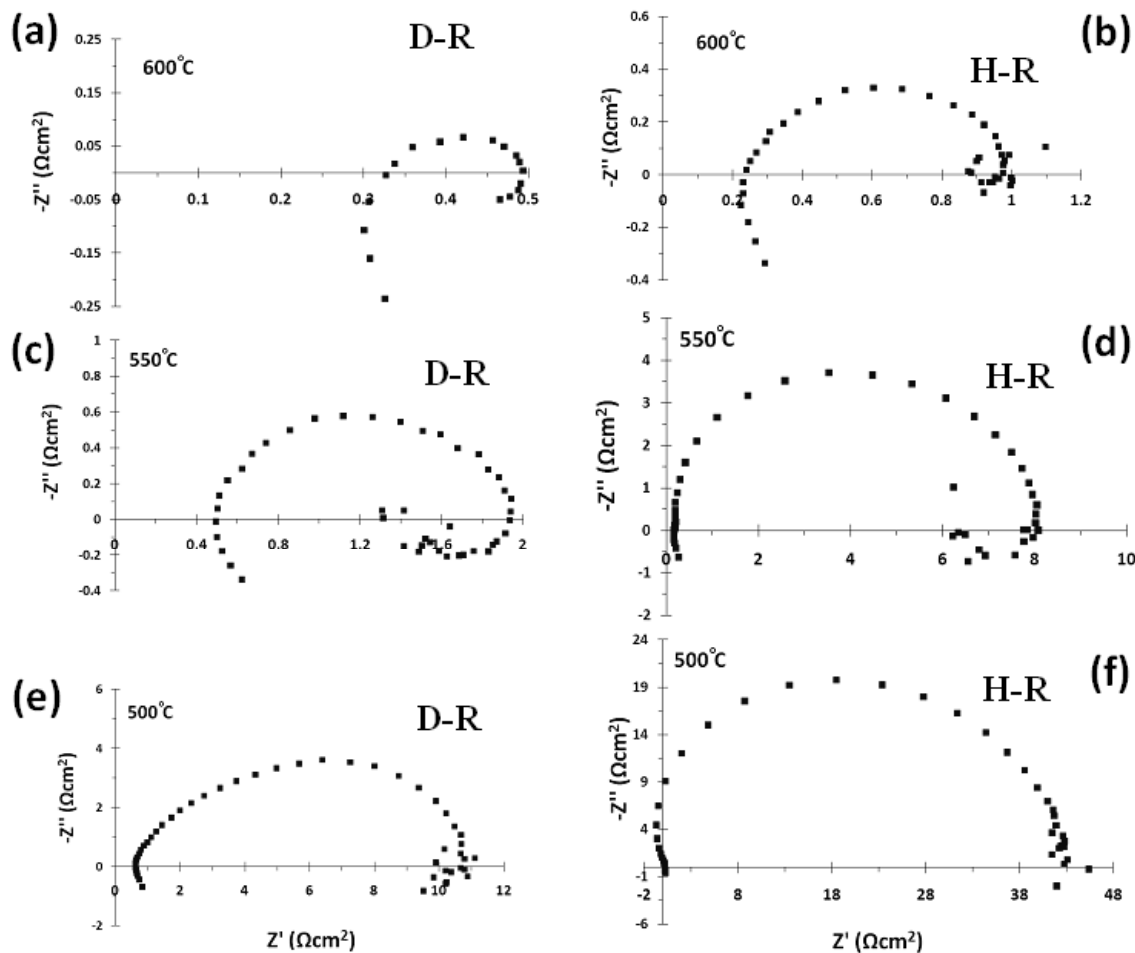
Fig. 4. Anodic impedance spectra for the H_2 oxidation reaction on the D-R and H-R anodes as a function of temperature in 97% H_2 /3% H_2O at open circuit.
